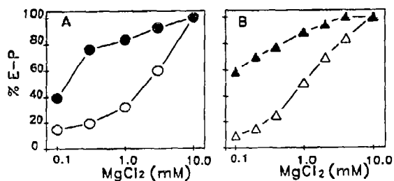
Fig. 3. Mg^{2+} dependence: Effects of a Ca^{2+} gradient and dimethyl sulfoxide. The assay medium composition was 50 mM MOPS-Tris buffer (pH 7.0), 5 mM EGTA, 1.0 mM (A) or 0.2 mM (B) ^{32}P_i , 0.1 mg/ml vesicle protein and MgCl_2 as indicated. The reaction was started by the addition of vesicles and arrested after 30 s at 35°C by the addition of 20% (w/v) TCA solution containing 2 mM P_i . (A) empty vesicles (no gradient) and (B) Ca^{2+} -loaded vesicles (gradient). (○, △) Totally aqueous medium; (●, ▲) 20% (v/v) dimethyl sulfoxide. In (A) 100% phosphoenzyme (E-P) was (○) 1.5 and (●) 2.6 \mu\text{mol/g} . In (B) 100% was (△) 1.3 and (▲) 2.7 \mu\text{mol/g} .
